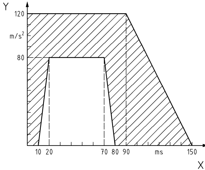
Figure 6 — Acceleration impulse
